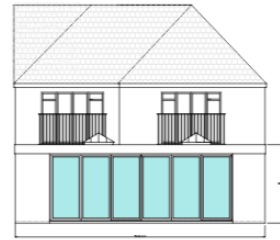
Rear Elevation Proposed
